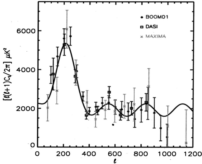
FIG. 1. Data from BOOMERanG, DASI and MAXIMA. Overplotted, our best fit from the class of models described by Eq. (3).
